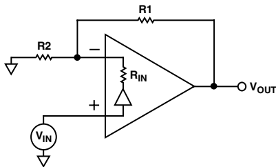
Figure 4. Follower with Gain
